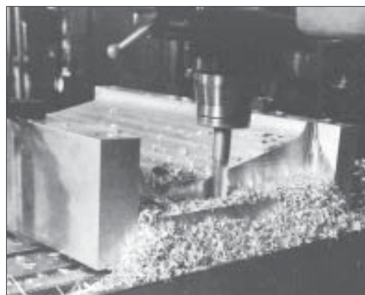
Milling Alumec 89.
